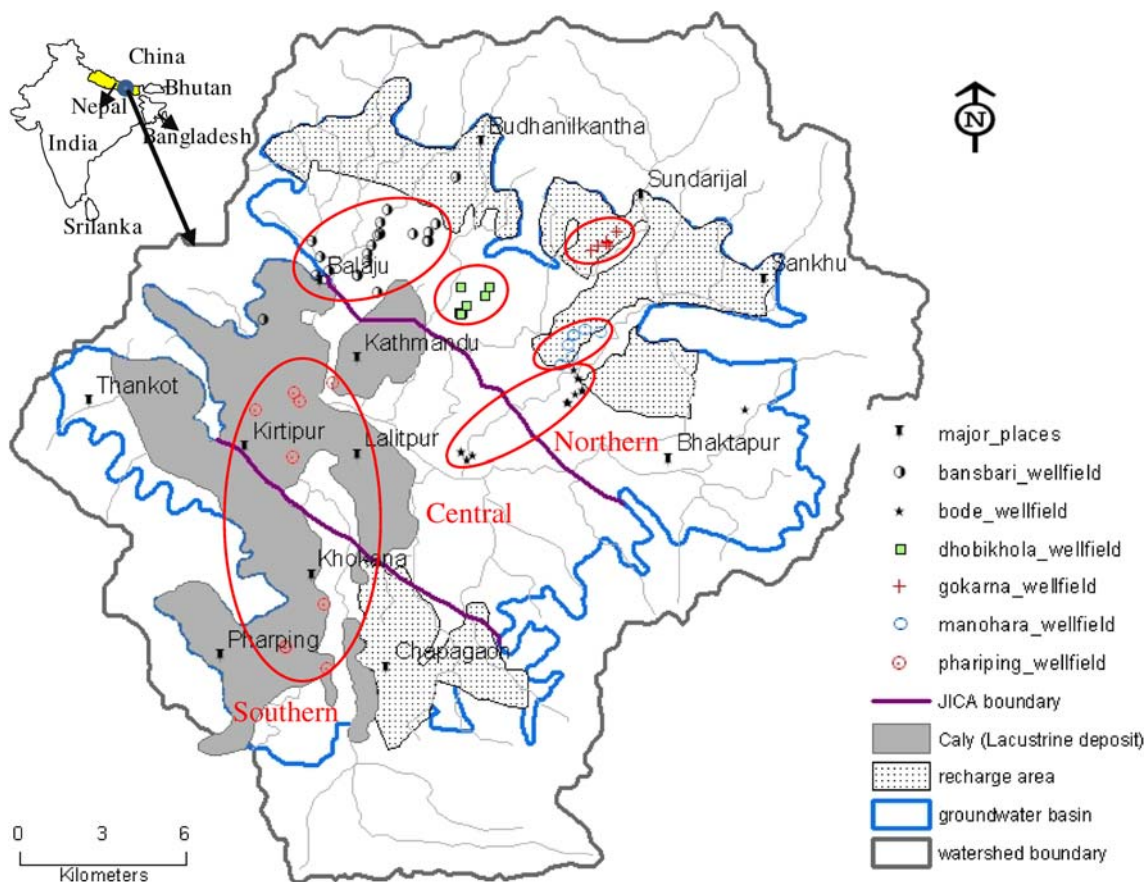
Fig. 1 Surface watersheds, groundwater basin, recharge areas and NWSC well-elds in Kathmandu Valley aquifer (Sources: groundwater basin boundary and recharge area (JICA 1990), clay deposit (Jha et al. 1997))
